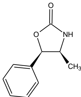
(4S,5R)-4-methyl-5-phenyl-2-oxazolidinone
