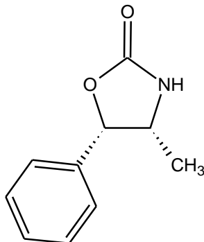
(4R,5S)-4-methyl-5-phenyl-2-oxazolidinone
